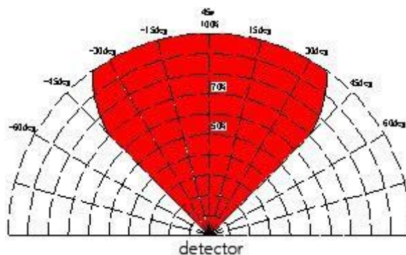
Figure 3-- Field view plan of infrared flame detector
